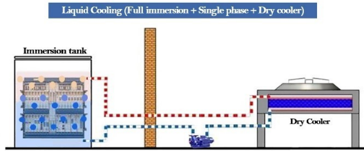
Figure 1: Single-phase Immersion Cooling Loop
